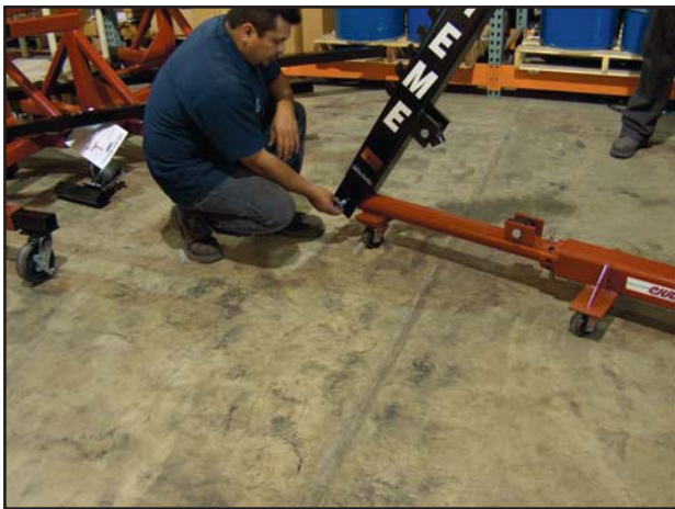
Attach Pulling Tower to Tower Base with supplied bolt. Tighten securely.
