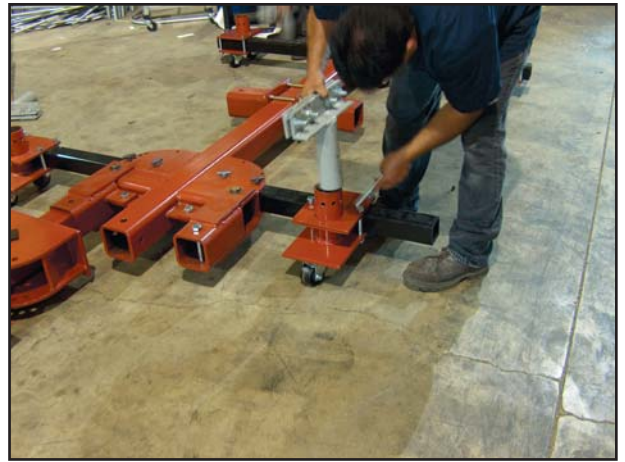
Install Pinchweld Clamps into Clamp Brackets. Insert Locking Pin to hold clamp into position. Height is adjustable.
