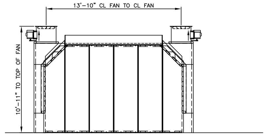
END VIEW
