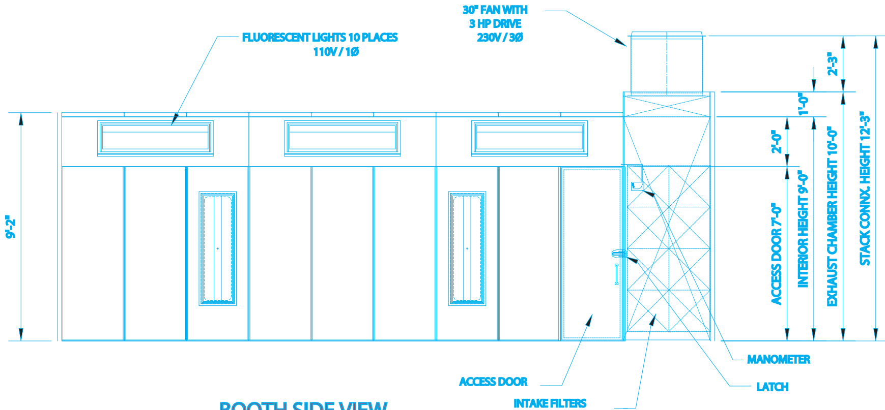
BOOTH SIDE VIEW
