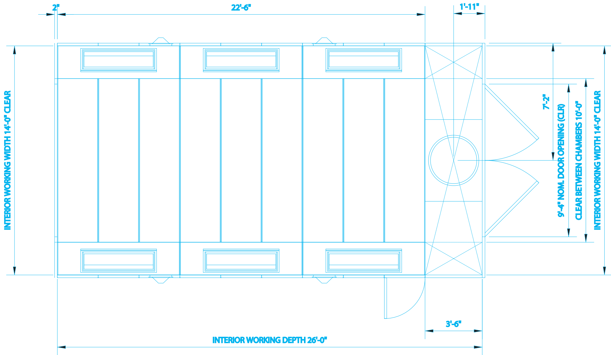
PLAN VIEW
